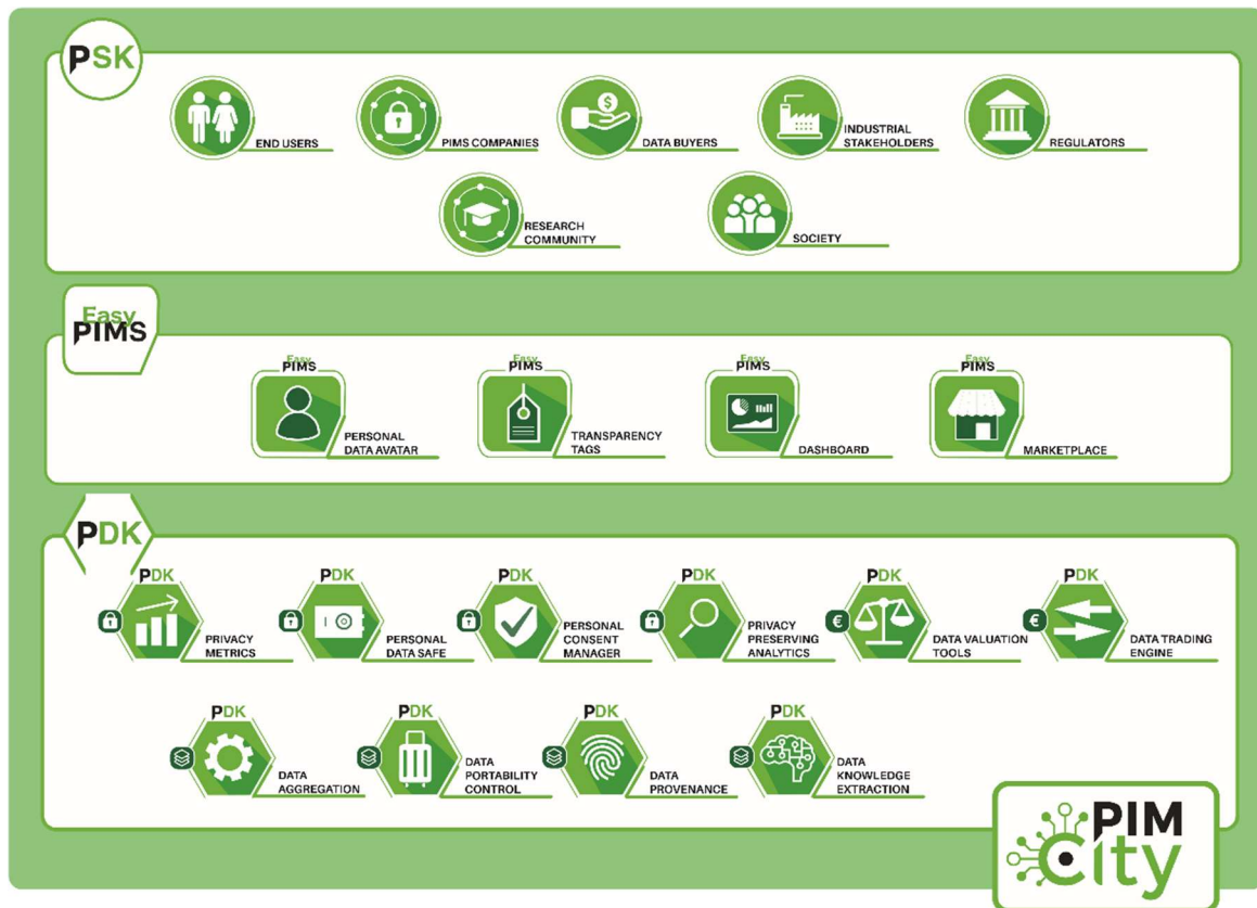
Figure 14: PIMCity components
